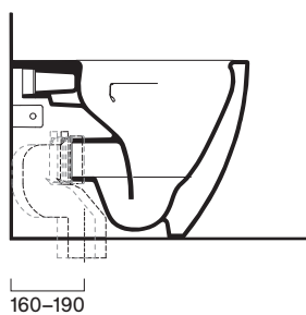
cod. 90 5455 0000 Adjustable pipe elbow fitting.
