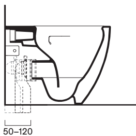
cod. 90 5457 0000 Adjustable pipe elbow fitting.
